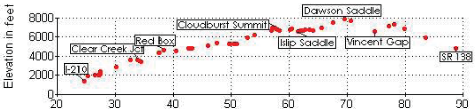
Angeles Crest Highway Elevation Profile
